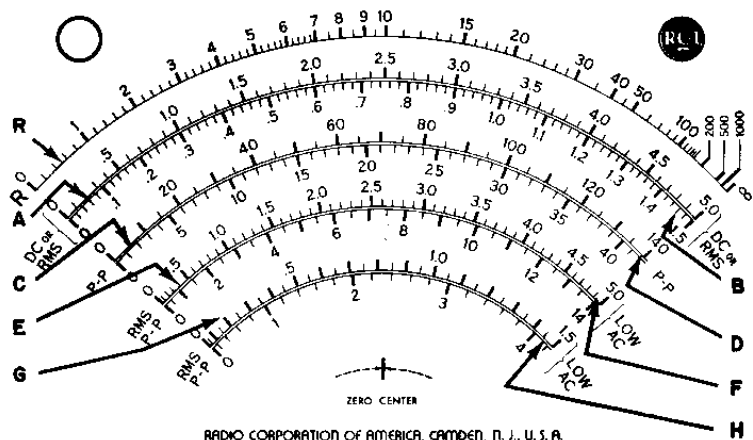
Figure 1. WV-98B meter scales
