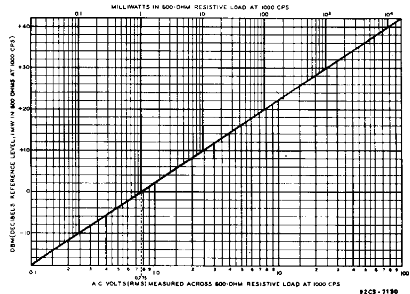
Figure 9. Graph for conversion of rms voltages to dbm values
