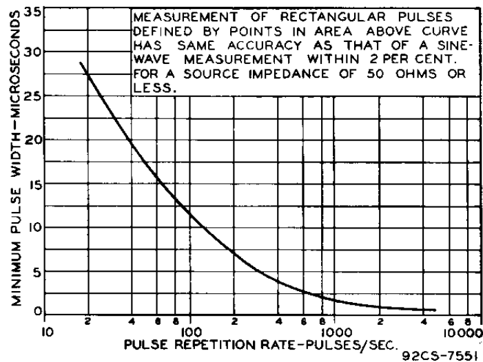
Figure 8. Pulse response capability of the WV-98B
