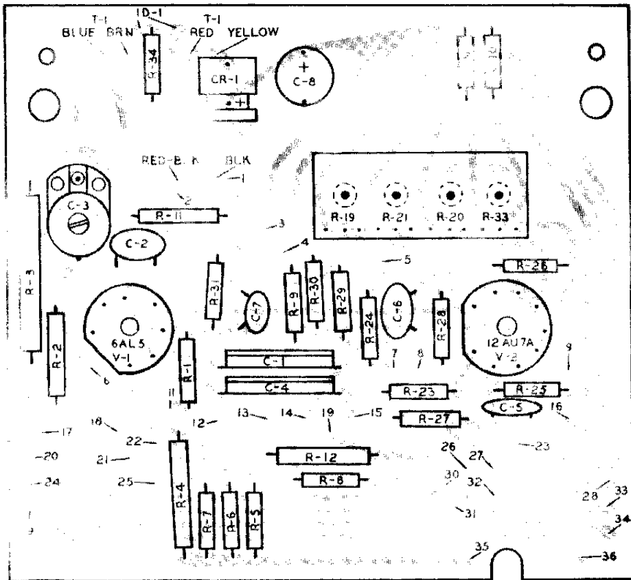
Figure 6. View of component side of laminated board, showing circuit contacts underneath
