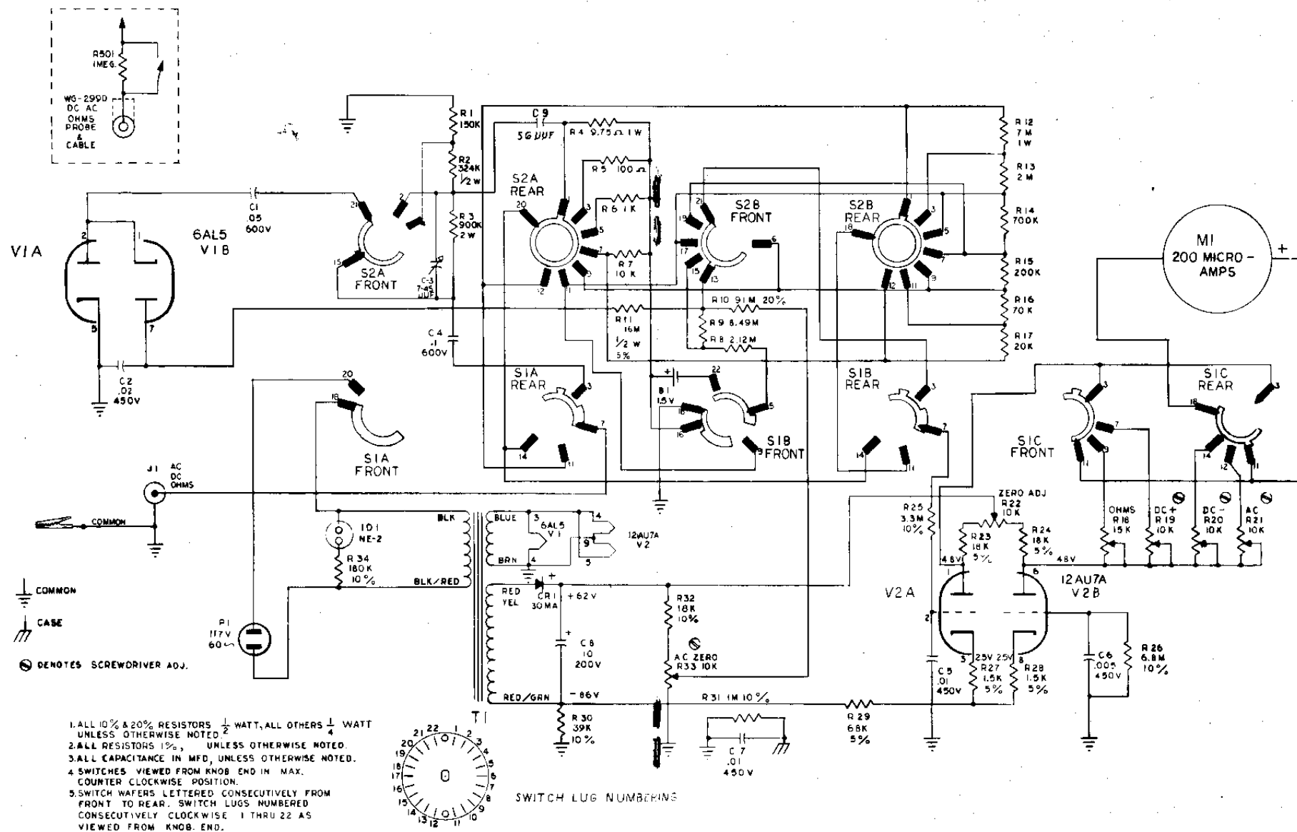
Figure 5. Schematic diagram of the WV-98B
